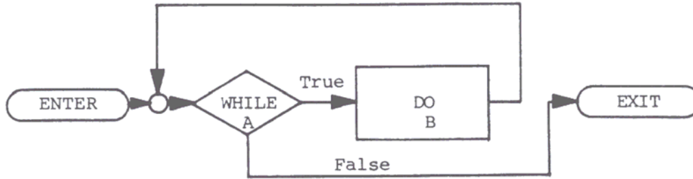
Figure 3 DO-WHILE
