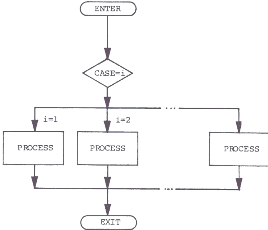
Figure 5 CASE
