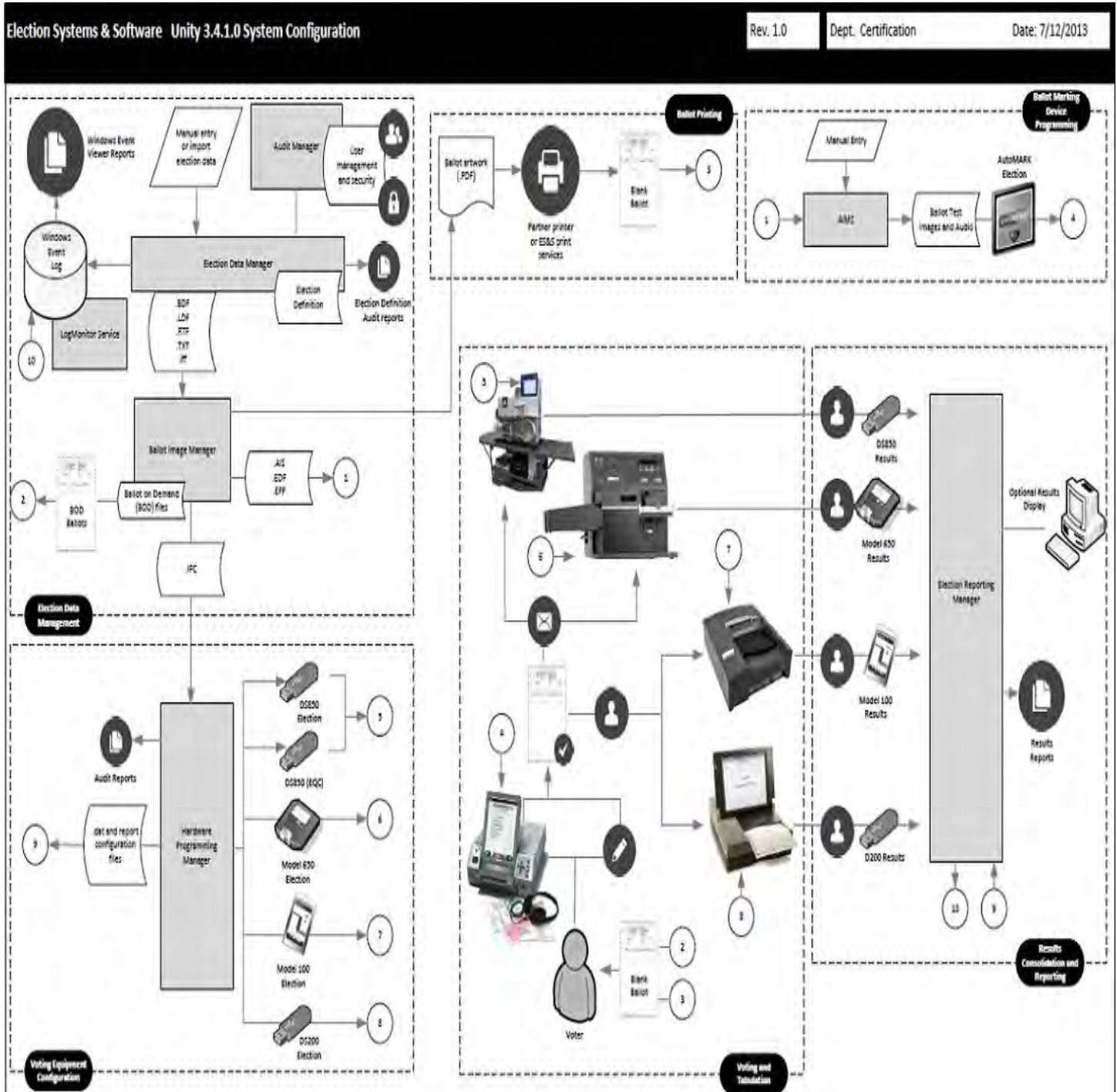
Figure 2-1 System Overview Diagram
