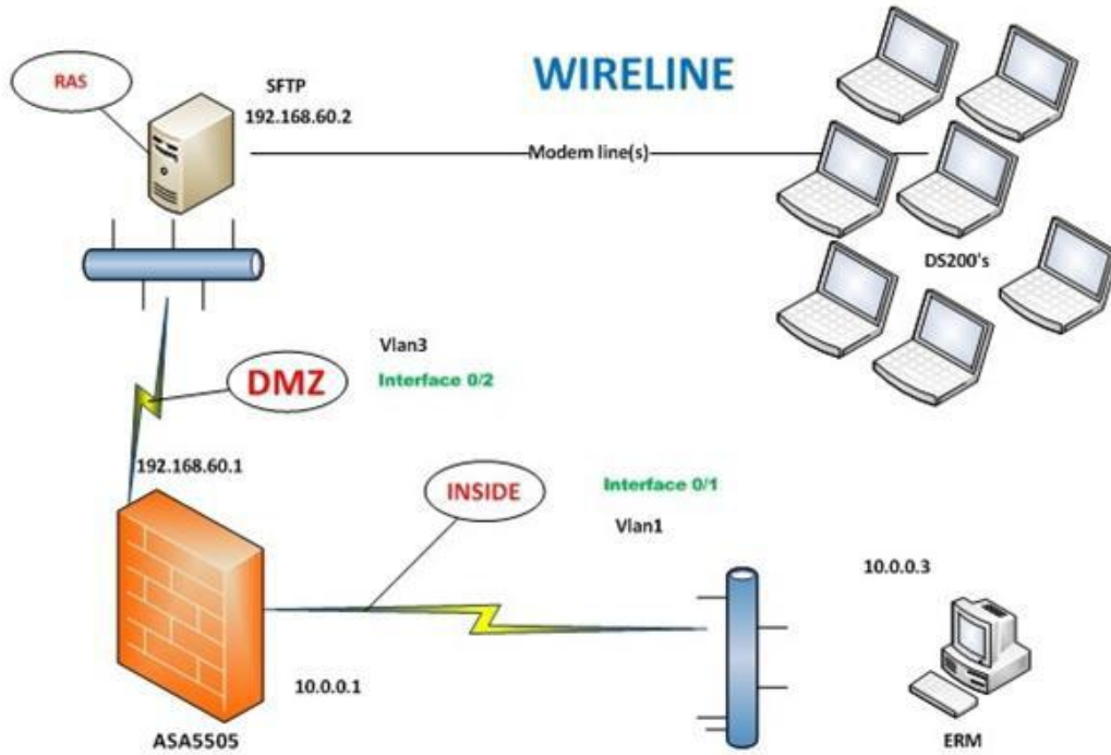
Figure 1-4 Wired Results Transmission Subsystem
